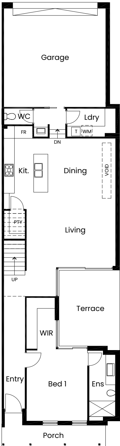
GROUND FLOOR
